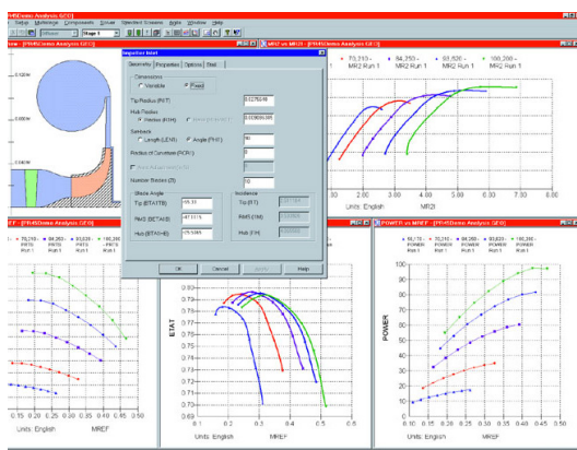
Multiple speed line performance map with IGV and volute.
