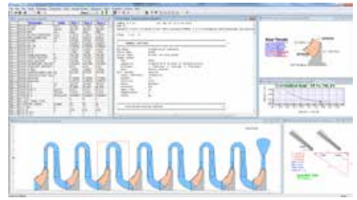
Multistage pump design example
